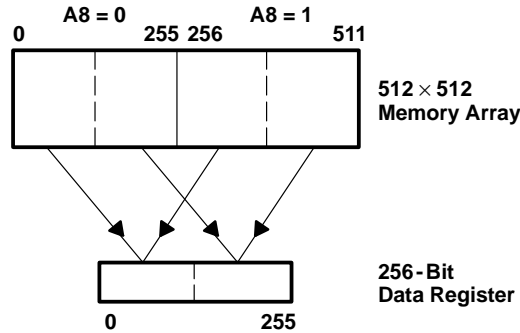
Figure 21. Split-Register-Transfer Read
