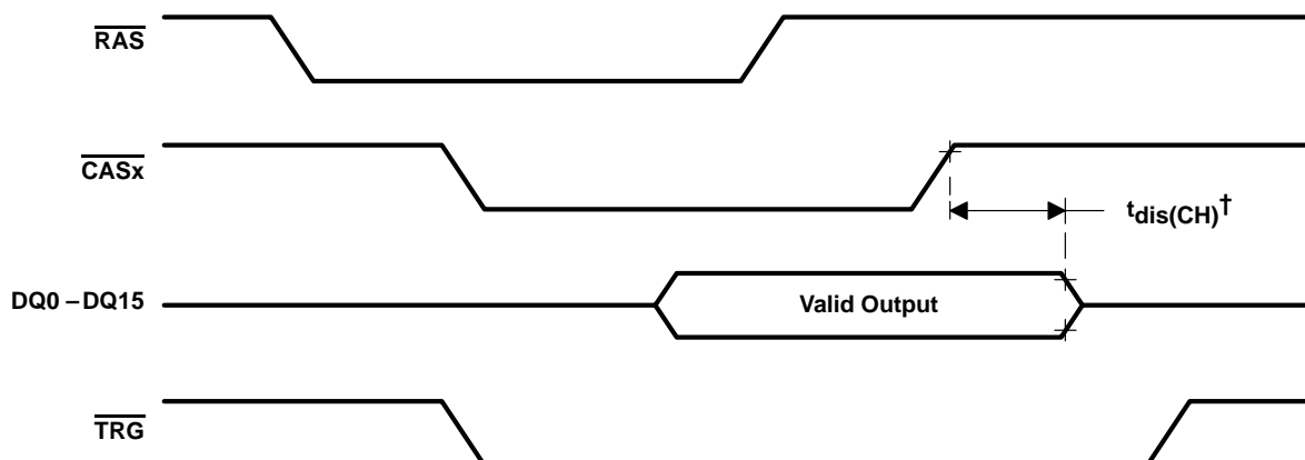
Figure 2. DRAM Read Cycle With \overline{CAS} -Controlled Output (TMS551x1)
