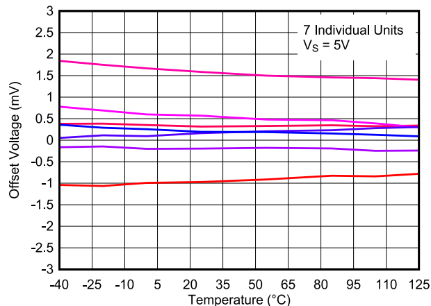
Figure 8-28. Offset Voltage vs. Temperature, 5 V
