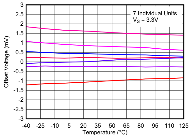
Figure 8-27. Offset Voltage vs. Temperature, 3.3 V
