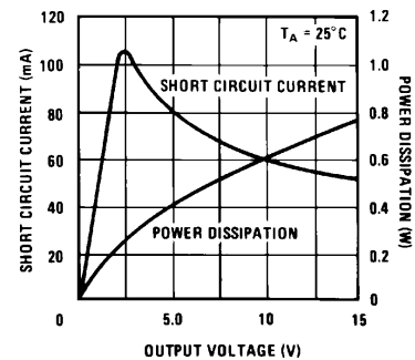
Figure 12. Output Limiting Characteristics
