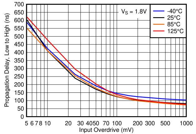
Figure 6-18. Propagation Delay, Low to High, 1.8V
