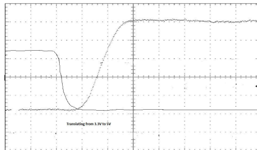
Figure 9-3. Up Translation
