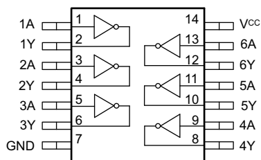
Figure 5-1. SN54AHCT04 J or W Package, 14-Pin (Top View)
