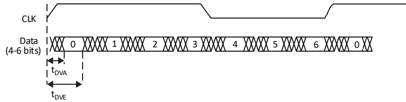
Figure 3.7. Receiver GDDR71_RX. Waveforms
