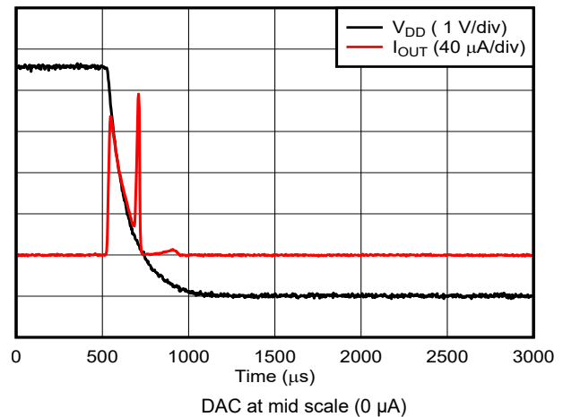
Figure 6-52. Current Output Power-Off Glitch
