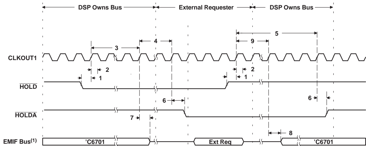
Figure 24. \overline{HOLD}/\overline{HOLDA} Timing
