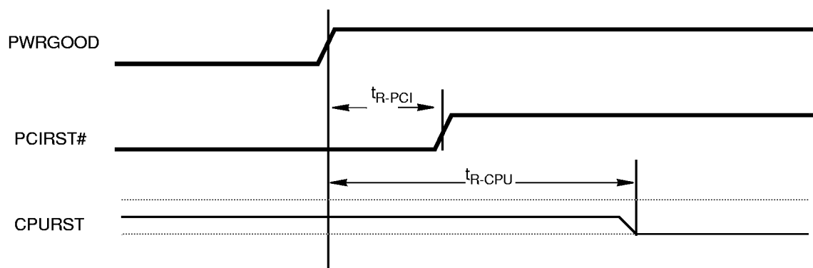
FIGURE 22. Reset Timing
