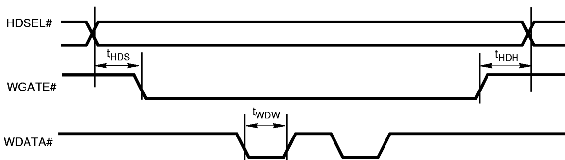
FIGURE 19. Write Data Timing
