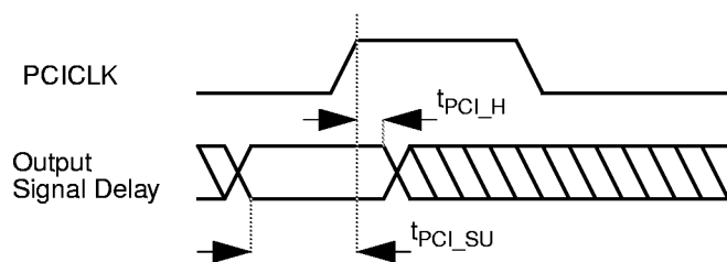
FIGURE 4. PCI Bus Input Signals
