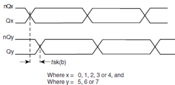
BANK SKEW
