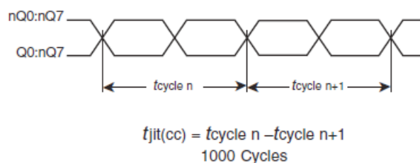
CYCLE-TO-CYCLE JITTER
