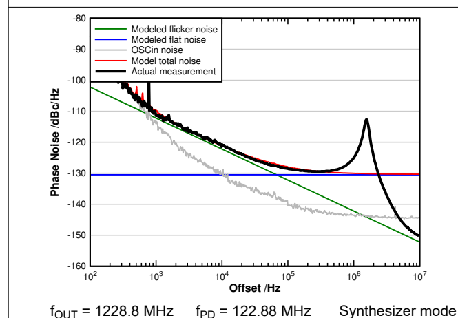
Figure 6-12. Normalized PLL 1/f Noise and Noise Floor
