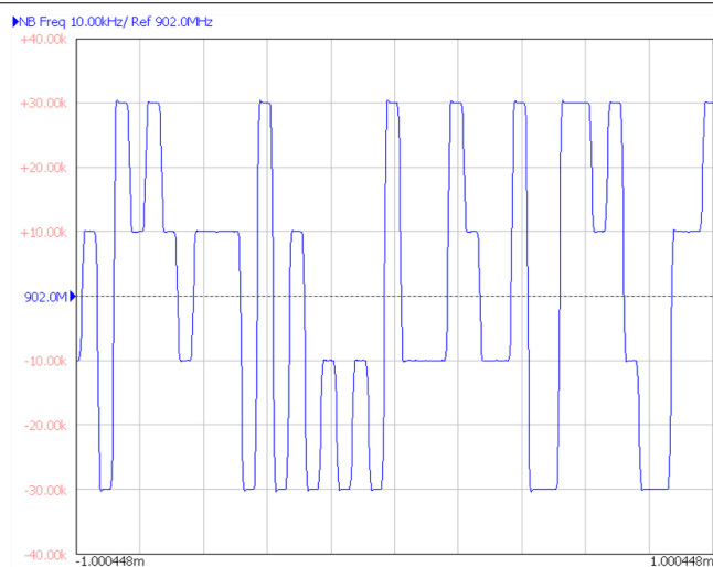
Figure 8-20. 4FSK Modulation
