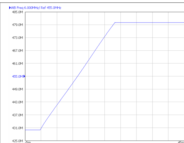
Figure 8-9. Change F1 Frequency Through SPI Programming
