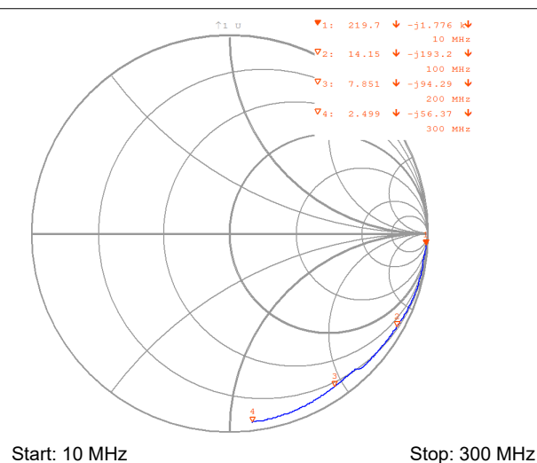
Figure 6-11. OSCin Input Impedance
