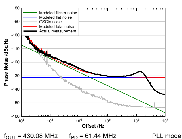
Figure 6-13. Normalized PLL 1/f Noise and Noise Floor
