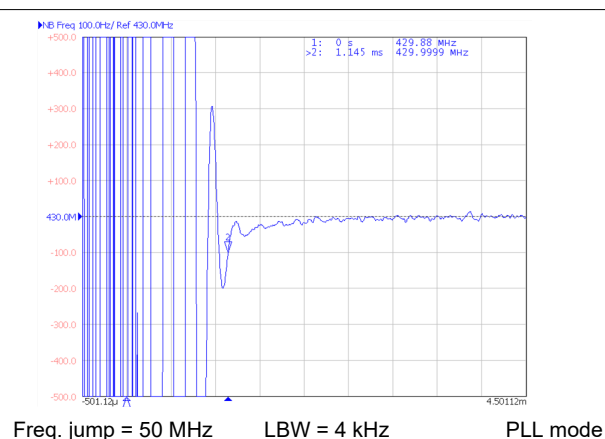
Figure 6-9. FastLock With SPST Switch
