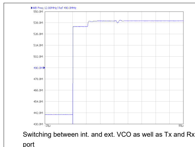
Figure 6-8. Output Port and VCO Switching
