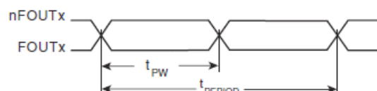
PERIOD JITTER
