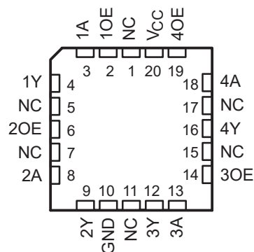
Figure 5-2. SN54AHCT126 FK Package, 20-Pin LCCC (Top View)
