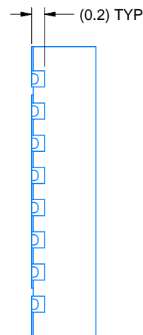
1.0 0.8 0.05 0.00 SEATING PLANE 0.08 C 1.05 0.95 2X 0.5 EXPOSED THERMAL PAD 14X 0.5 9 10 11 12 2X 3.5 3.05 2.95 2 19 20X 0.3 0.2 PIN 1 ID (OPTIONAL) 1 20 20X 0.45 0.35 ⌀ 0.1 C A B 0.05
