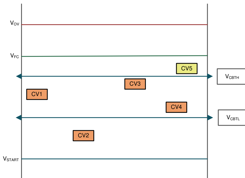
Figure 9-2. Cell-Balancing Algorithm
