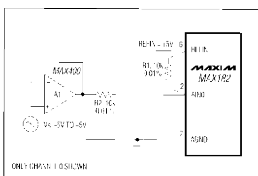
Figure 14. Bipolar -5V to +5V Operation
