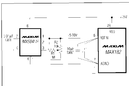
Figure 19. MAX5841H as Reference Generator
