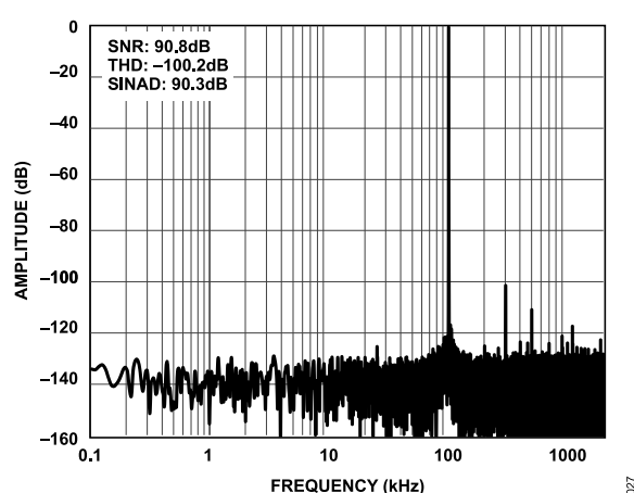
Figure 27. 100 kHz, -0.5 dBFS Input tone FFT, Gain = 0.3, Differential Input, Full Power
