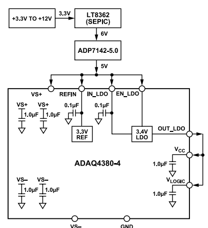
Figure 65. ADAQ4380-4 Power Supply Recommendations
