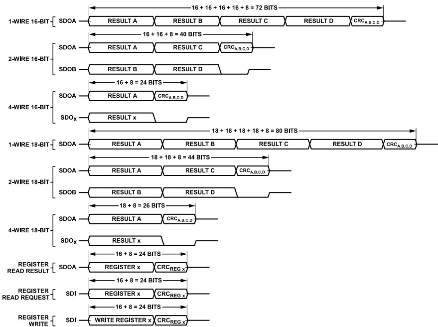
Figure 78. CRC Operation
