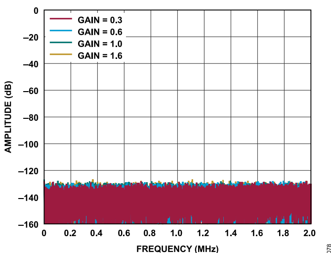
Figure 79. FFT with Shorted Inputs
