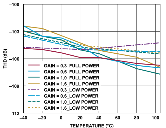
Figure 38. THD vs. Temperature, f_{IN} = 1 kHz
