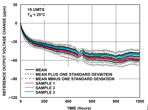
Figure 61. ADAQ4380-4 Internal Reference Long-Term Drift
