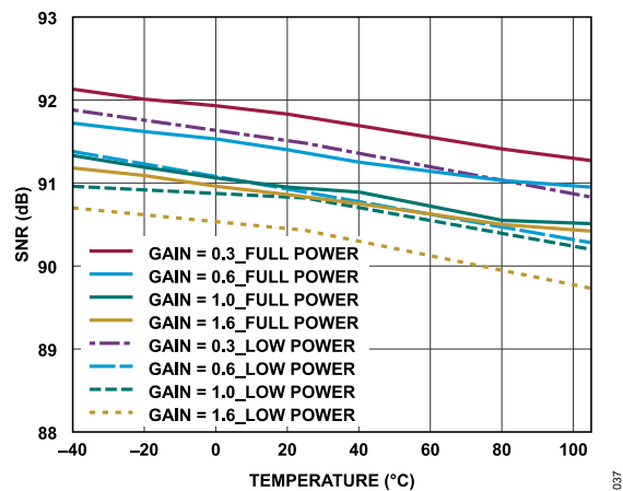
Figure 37. SNR vs. Temperature, f_{IN} = 1 kHz
