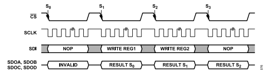
Figure 77. Register Write
