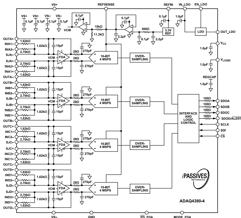
Figure 46. ADAQ4380-4 μModule Simplified Block Diagram
