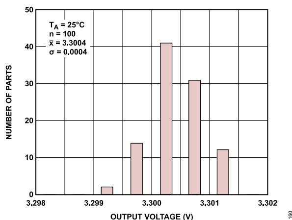
Figure 60. ADAQ4380-4 Internal Reference Output Voltage Accuracy
