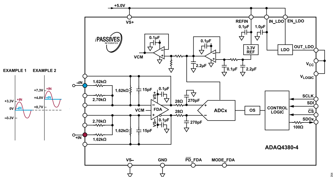
Figure 54. Single-Ended Input Configuration with Gain = 1.0, \pm 3.3 V Input, V_S = 5 V
