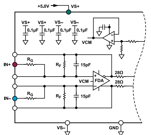
Figure 58. ADAQ4380-4 Configured at Fully Differential Inputs
