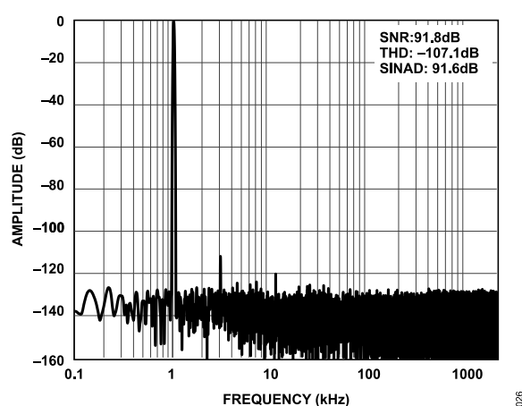
Figure 26. 1 kHz, -0.5 dBFS Input tone FFT, Gain = 0.3, Single-Ended Input, Full Power
