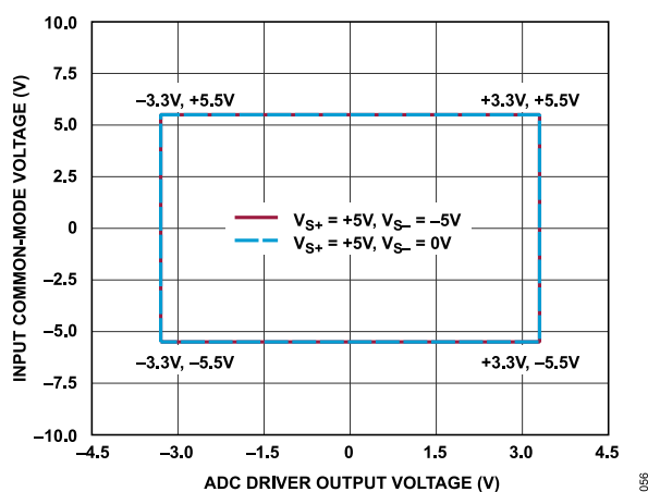
Figure 56. Input Common-Mode Voltage vs. ADC Driver Output, Gain = 0.3, \pm 11 V Differential Input
