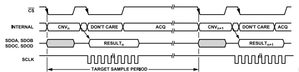
Figure 75. Low Throughput and Low Latency
