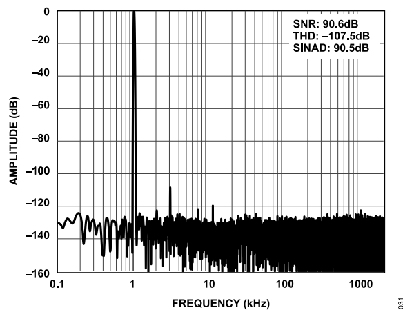
Figure 31. 1 kHz, -0.5 dBFS Input tone FFT, Gain = 0.6, Single-Ended Input, Low Power
