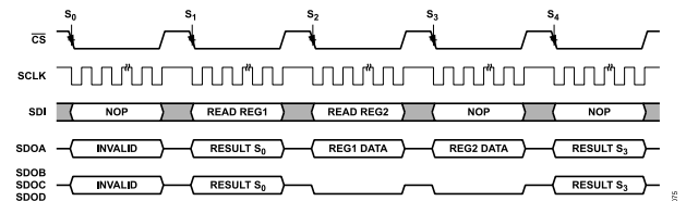
Figure 76. Register Read
