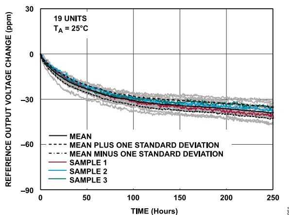
Figure 62. ADAQ4380-4 Internal Reference Early Life Drift
