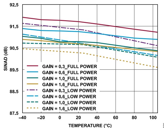
Figure 39. SINAD vs. Temperature, f_{IN} = 1 kHz
