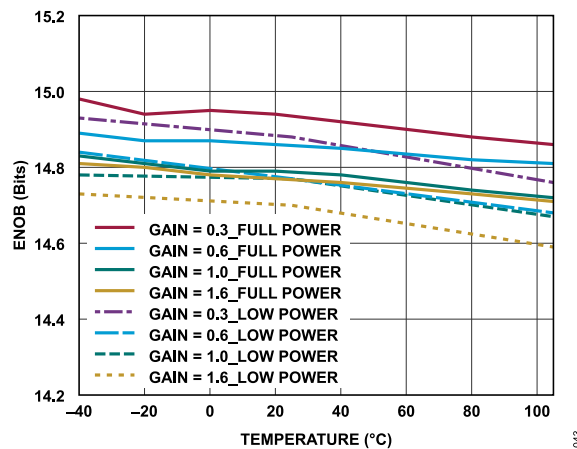
Figure 43. ENOB vs. Temperature, f_{IN} = 1 kHz
